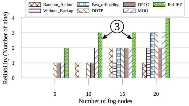
(c) Reliability with different numbers of fog nodes
