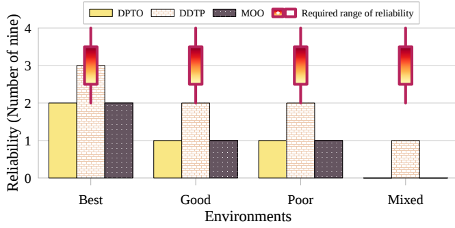
Fig. 1: Motivational example of a factory that needs a specific range of reliability levels in different environmental situations. In this example, DPTO, DDTP, and MOO are compared with the same number of tasks for 1500 times, and the average result is reported. The terms "Best," "Good," "Poor," and "Mixed" refer to fog node conditions with varying degrees of failure rate.
