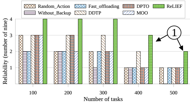
(a) Average reliability for different number of tasks.
