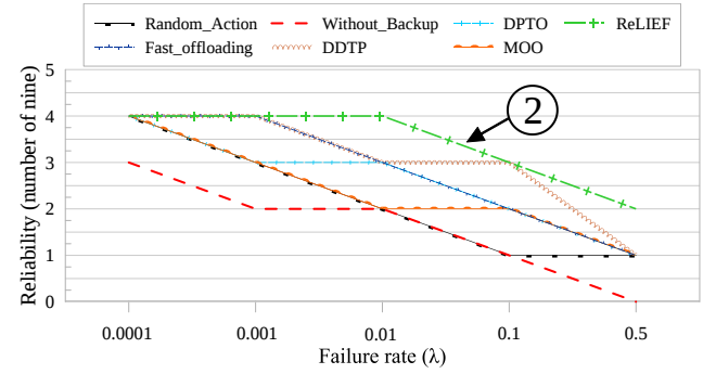
(b) Average reliability for different fault rates.
