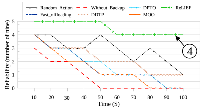
(d) Average reliability during 100 seconds with \lambda = 0.0001 .
